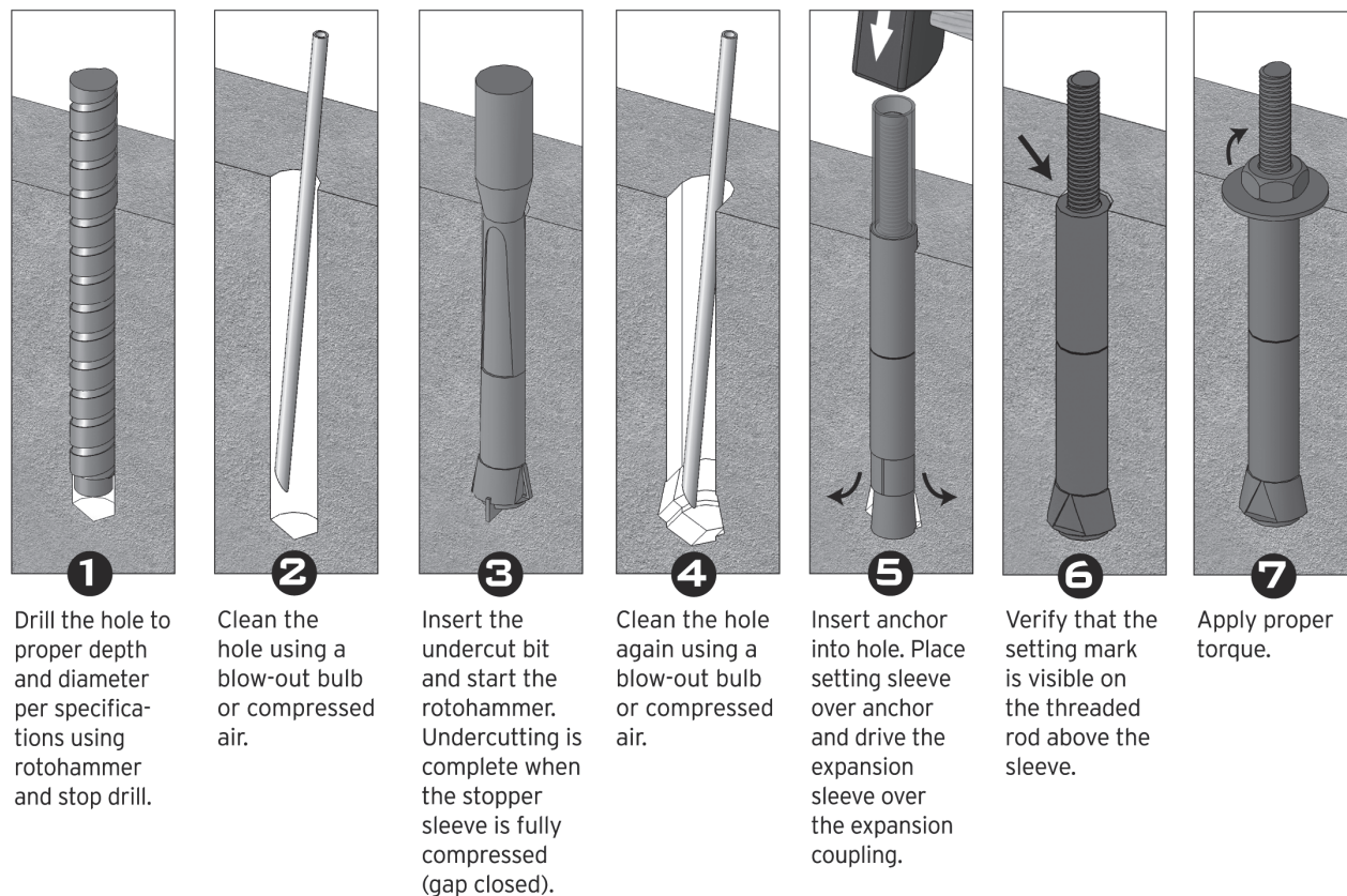
FIGURE 2—INSTALLATION OF DUC UNDERCUT ANCHOR
